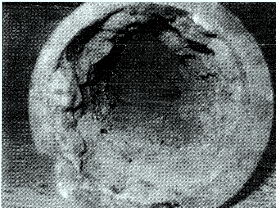
Figure 2 - Unlined cast iron pipe, with effects of corrosion shown, taken from within the Harmon Water Main Replacement Project area in the Village, 2005
