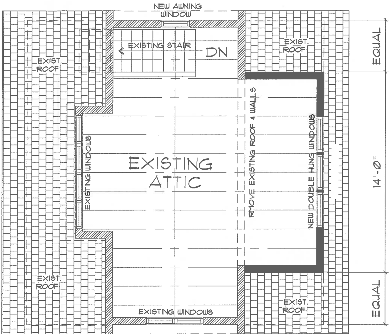
ATTIC LEVEL PLAN
