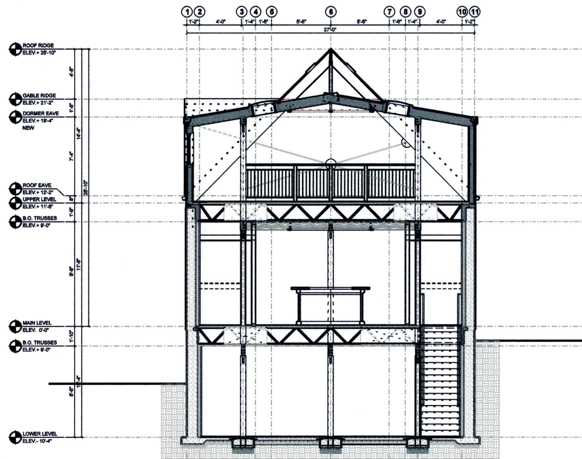
2 BUILDING CROSS SECTION - MIDDLE SCALE: 3/16" = 1'-0"
