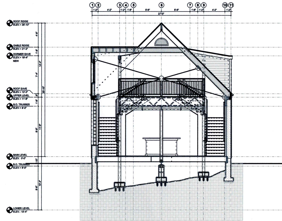
1 BUILDING CROSS SECTION - FRONT SCALE: 3/16" = 1'-0"
