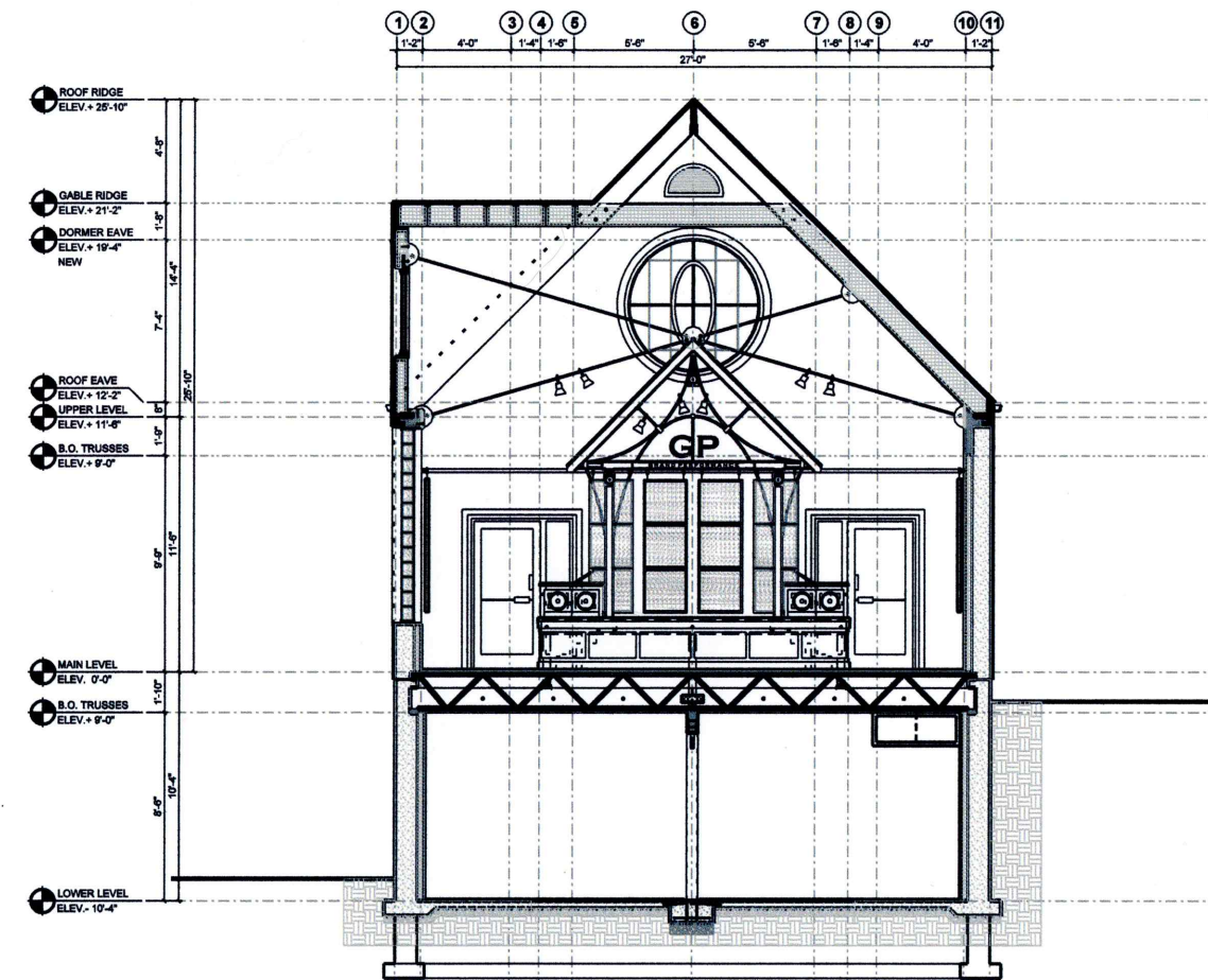
3 BUILDING CROSS SECTION - BACK SCALE: 3/16" = 1'-0"
