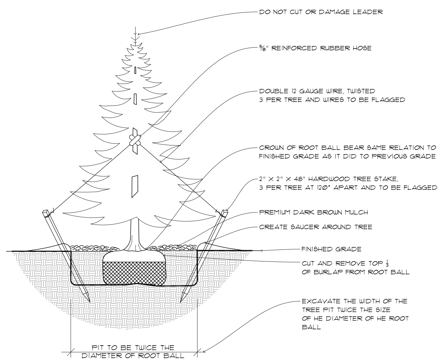
1 EVERGREEN PLANTING DETAIL LP-10 NTS
