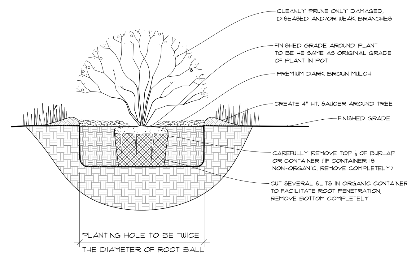
1 SHRUB PLANTING LP-10 NTS
