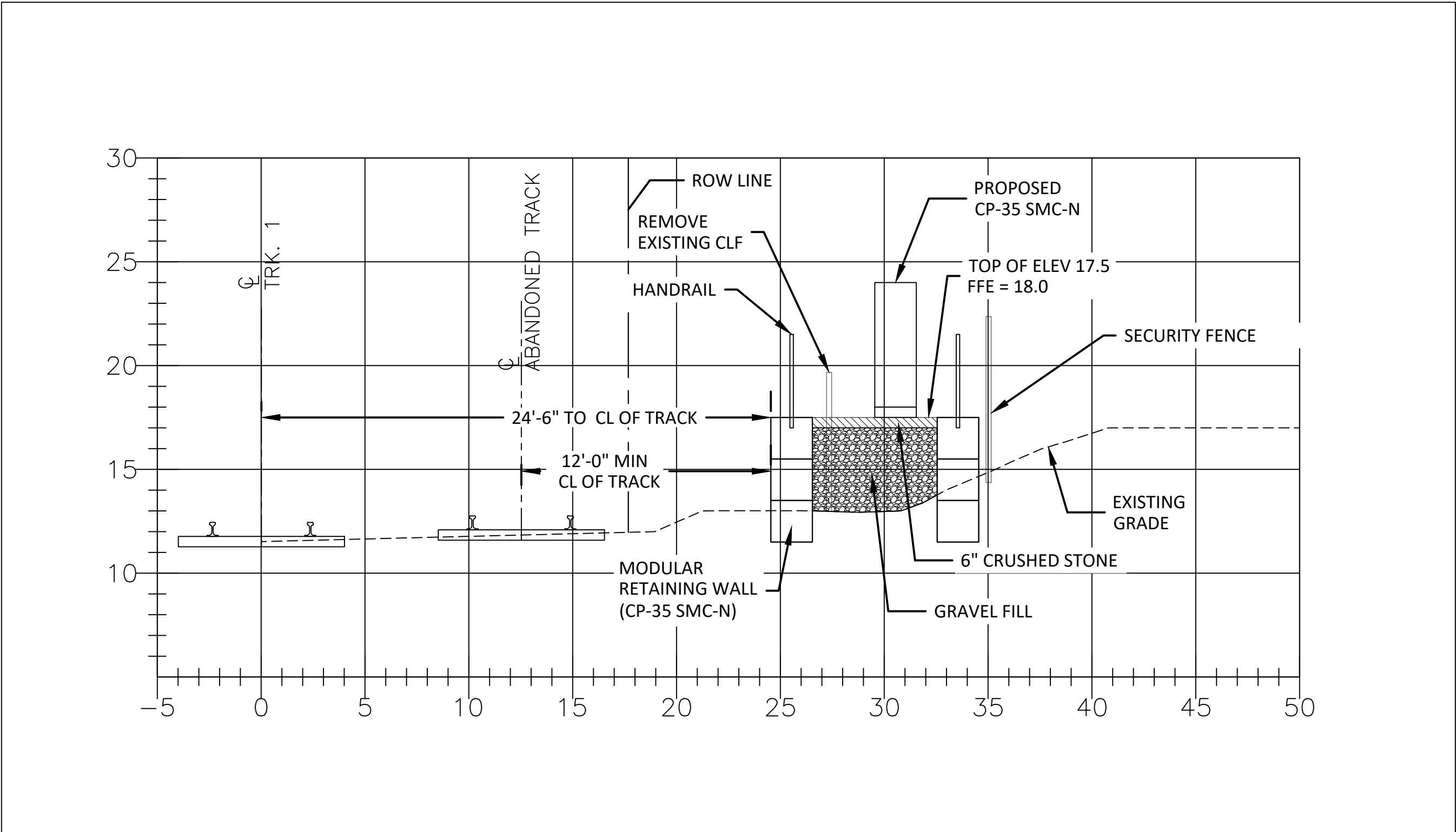
CP-35 SMC-N GRADING ELEVATION VIEW SCALE: 1" = 5'-0" 5' 2.5' 0 5' 10' 1" = 5'-0"
