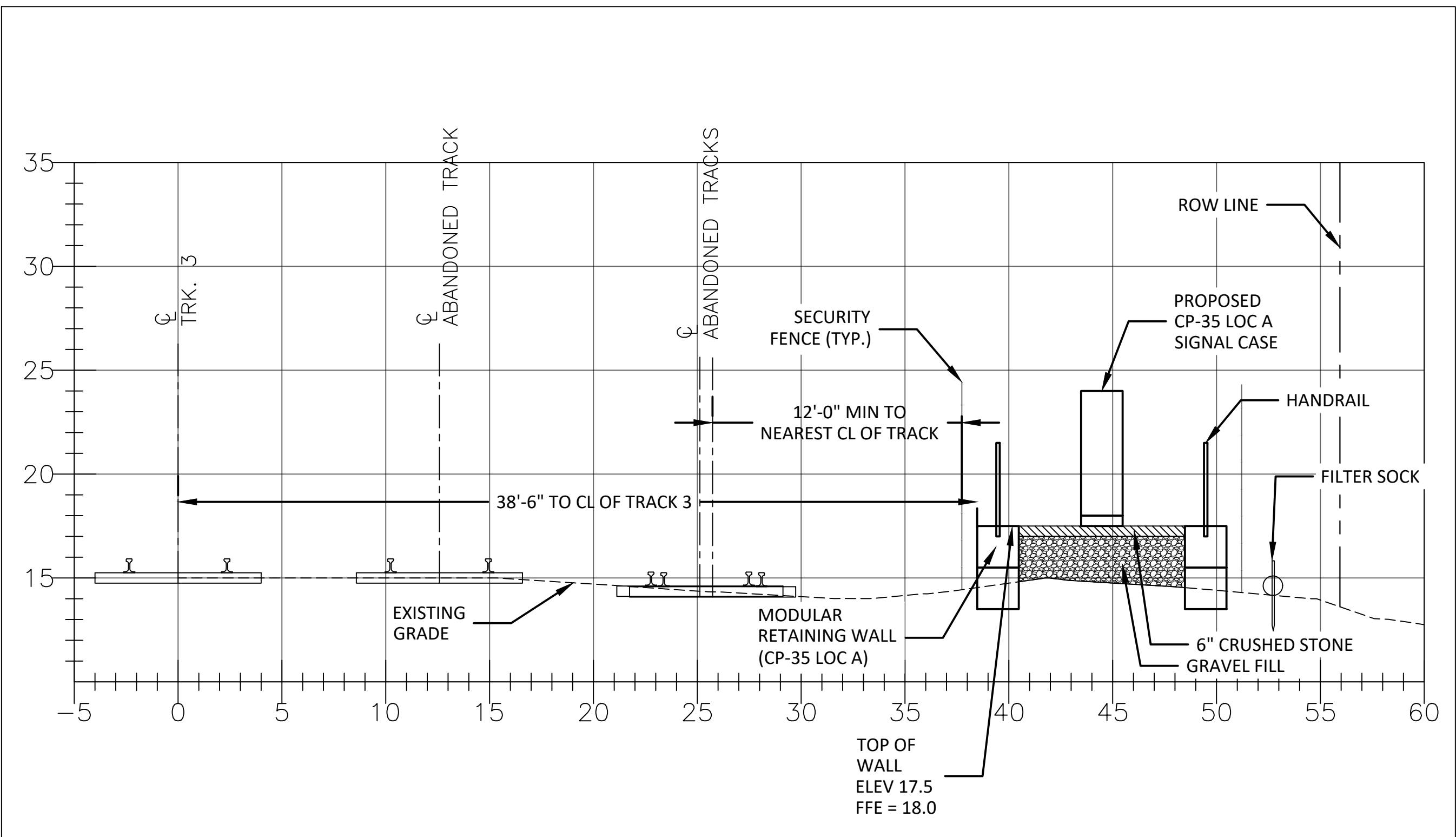
CP-35 LOC A GRADING ELEVATION VIEW
