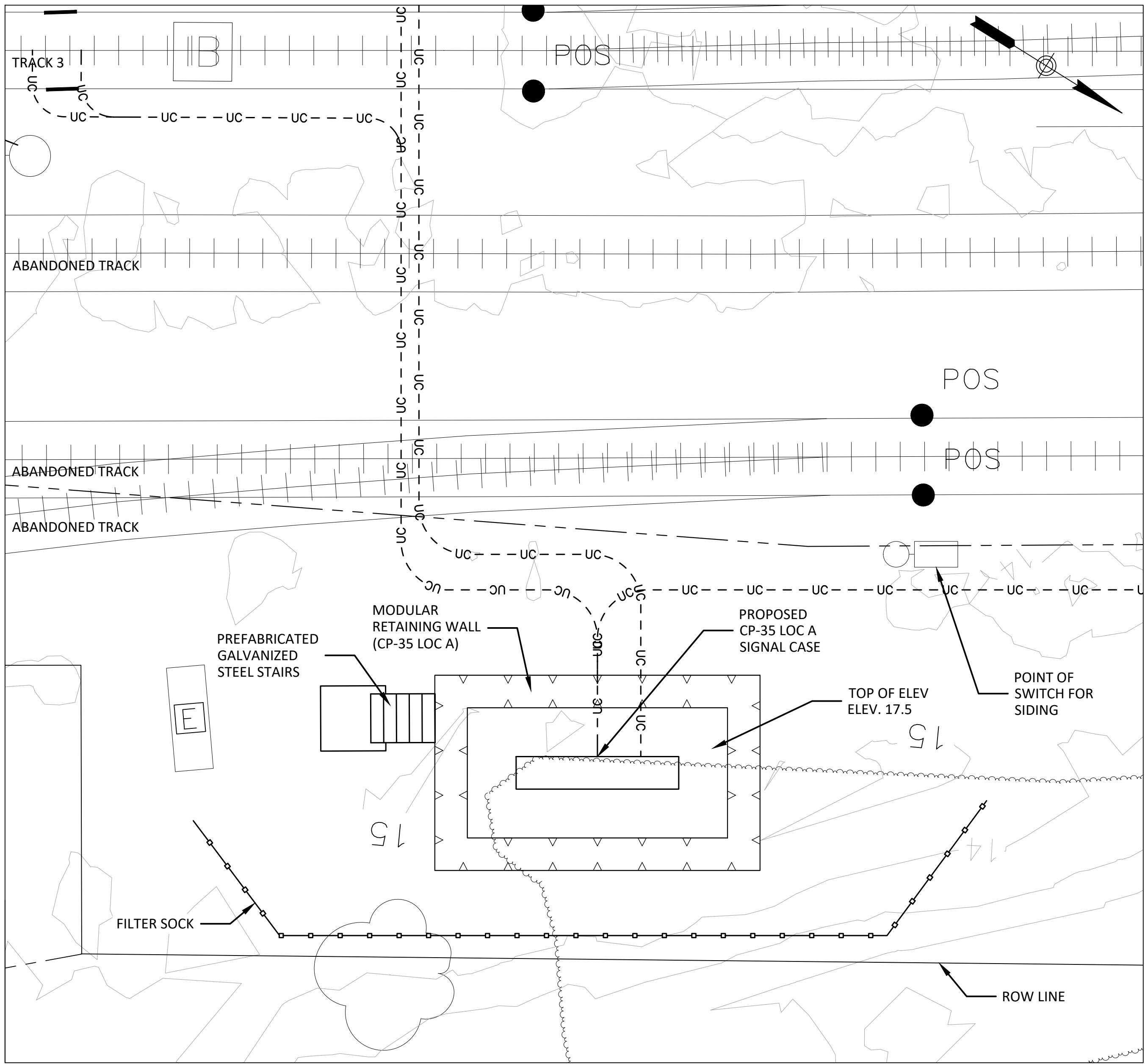
CP-35 LOC A GRADING PLAN VIEW
