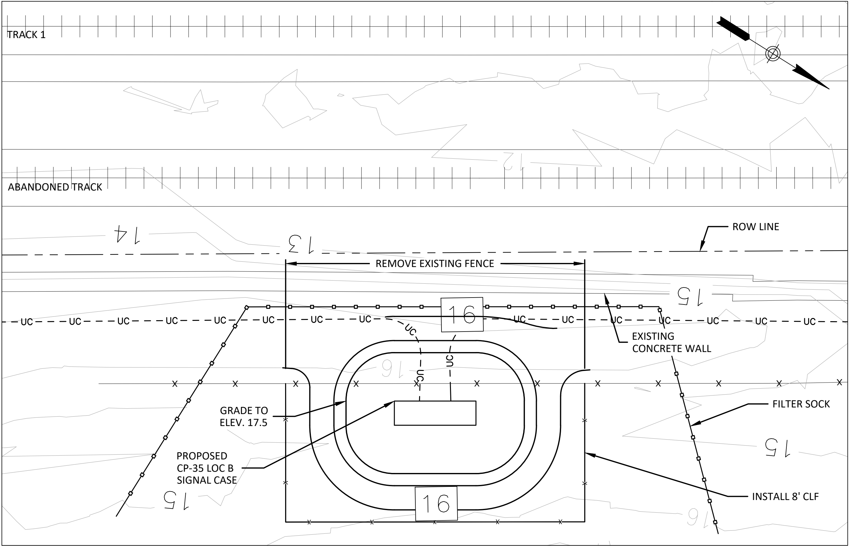
CP-35 LOC B GRADING PLAN VIEW
