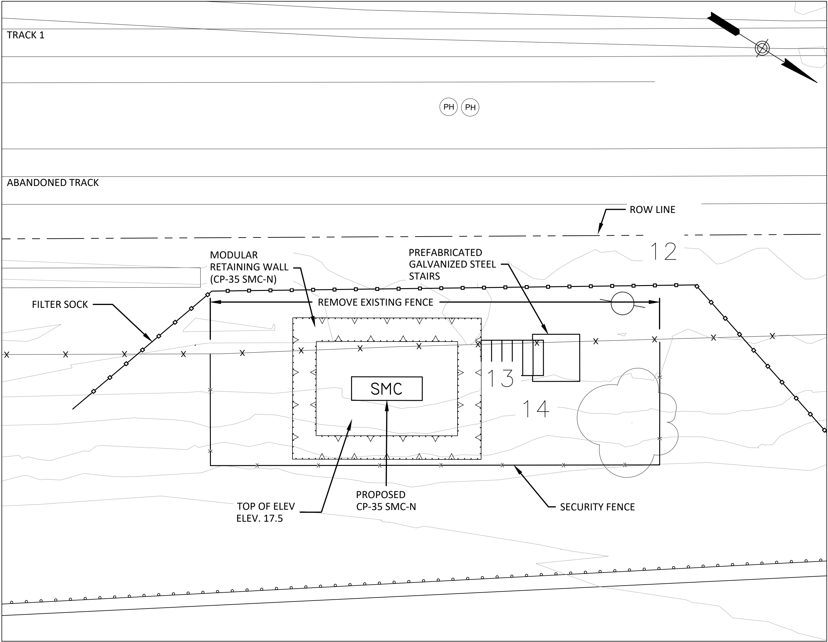
CP-35 SMC-N GRADING PLAN VIEW SCALE: 1" = 5'-0" 5' 2.5' 0 5' 10' 1" = 5'-0"
