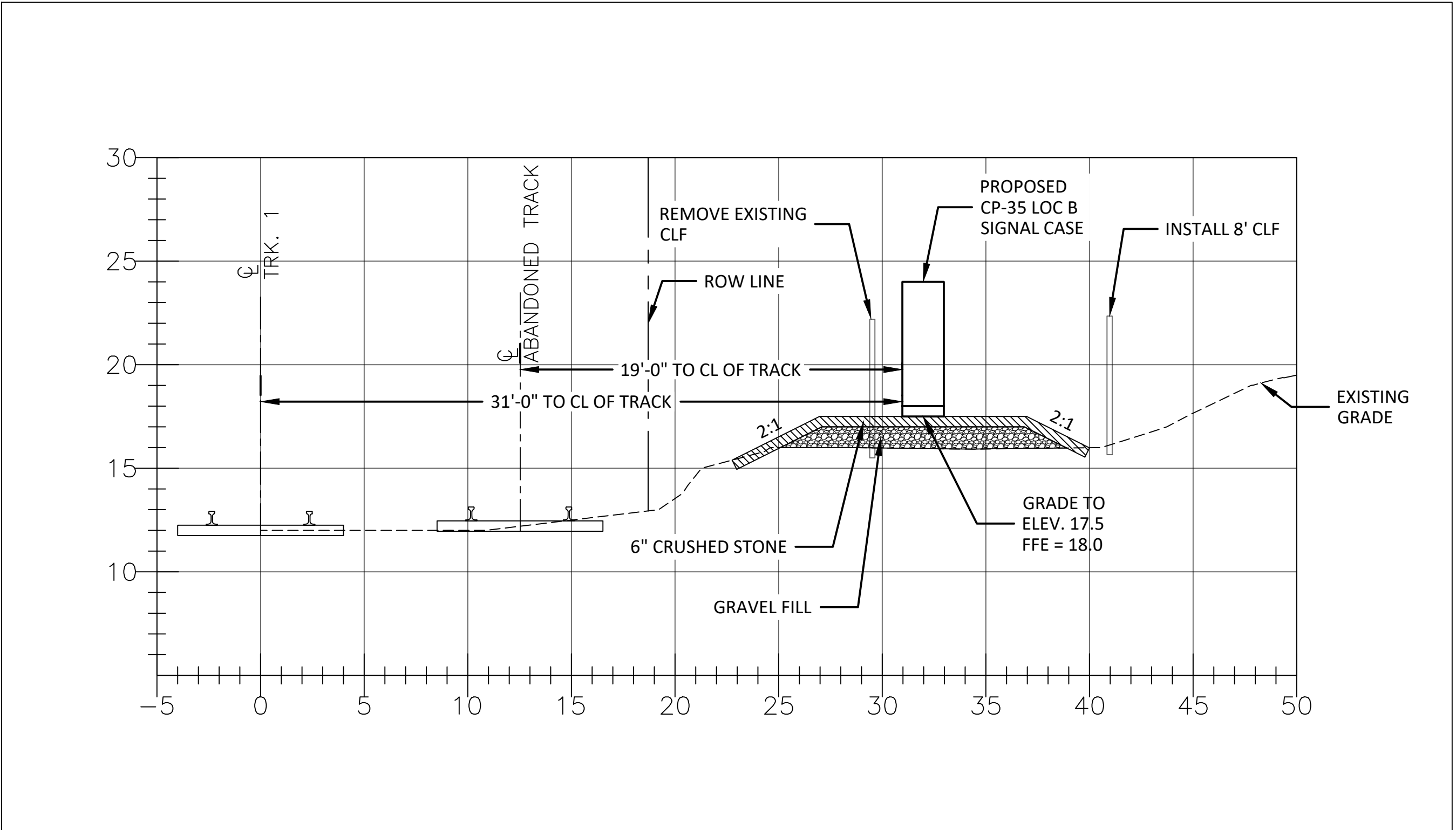
CP-35 LOC B GRADING ELEVATION VIEW
