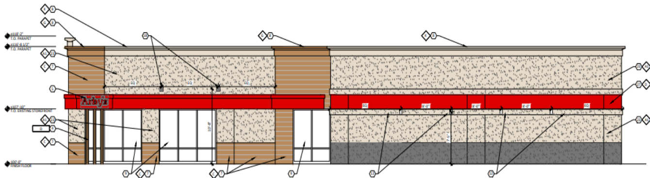
2 A2.2 EXTERIOR ELEVATIONS - EAST 1/4" = 1'-0"
