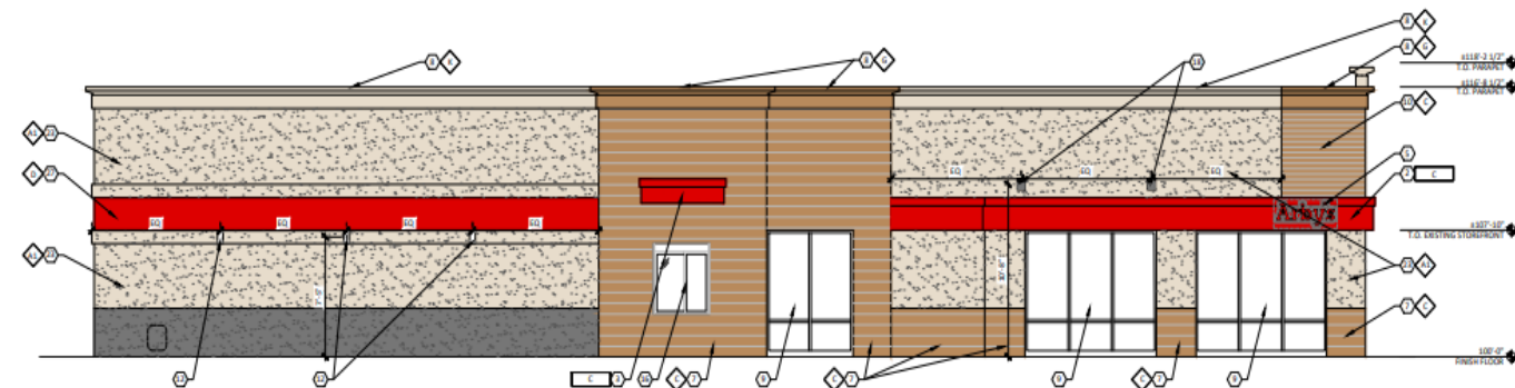
2 A2.1 EXTERIOR ELEVATIONS - WEST 1/4" = 1'-0"
