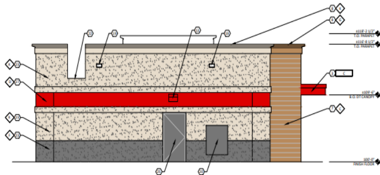
1 A2.2 EXTERIOR ELEVATION - NORTH 1/4" = 1'-0"
