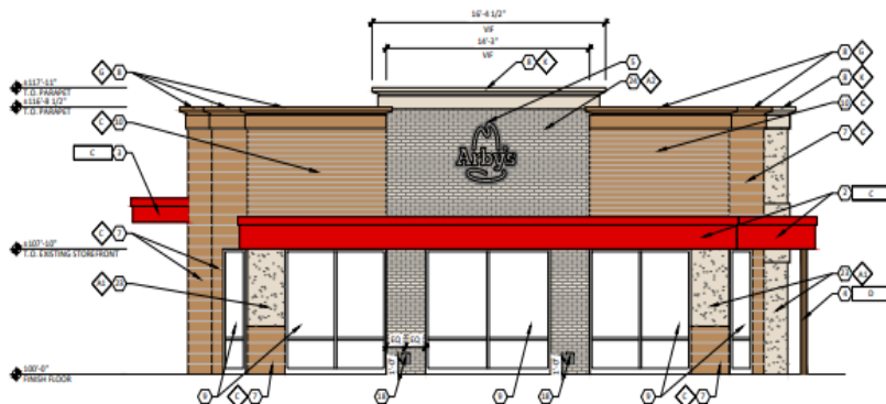
1 A2.1 EXTERIOR ELEVATION - SOUTH 1/4" = 1'-0"
