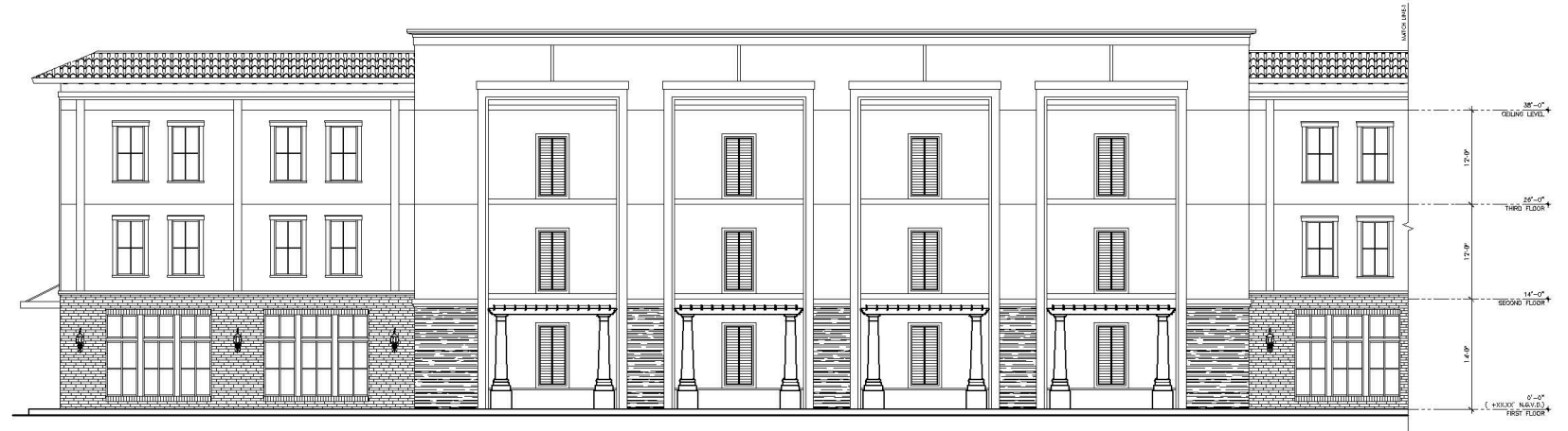
STORAGE BUILDING- SOUTH ELEVATION 1/8" = 1'-0"
