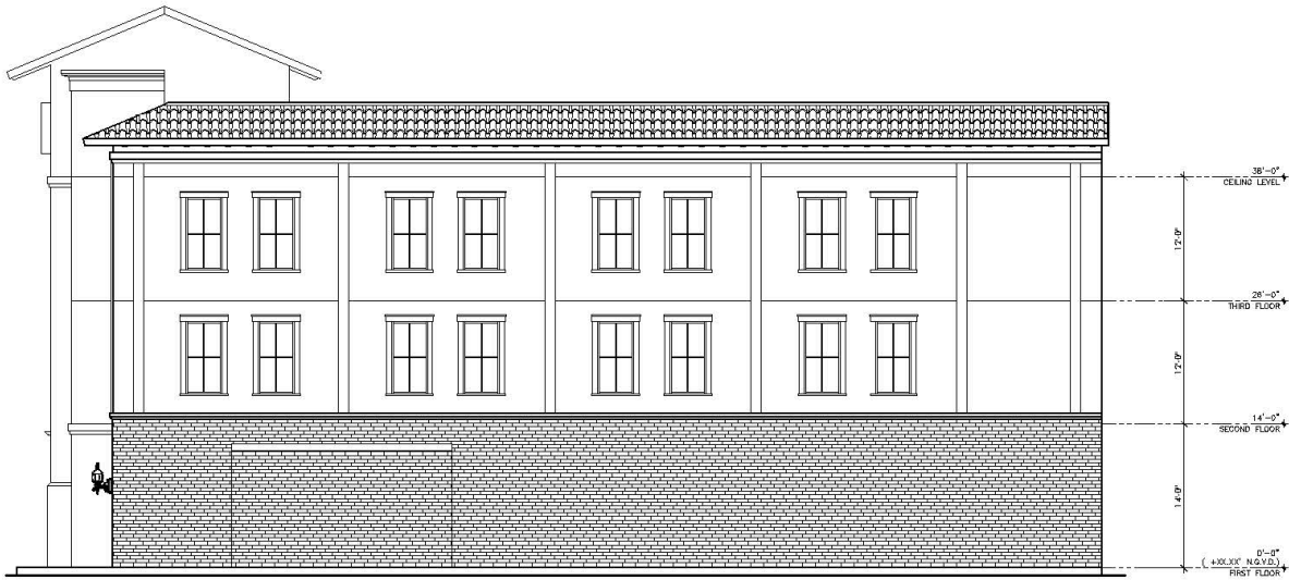
STORAGE BUILDING - EAST ELEVATION 1/8" = 1'-0"
