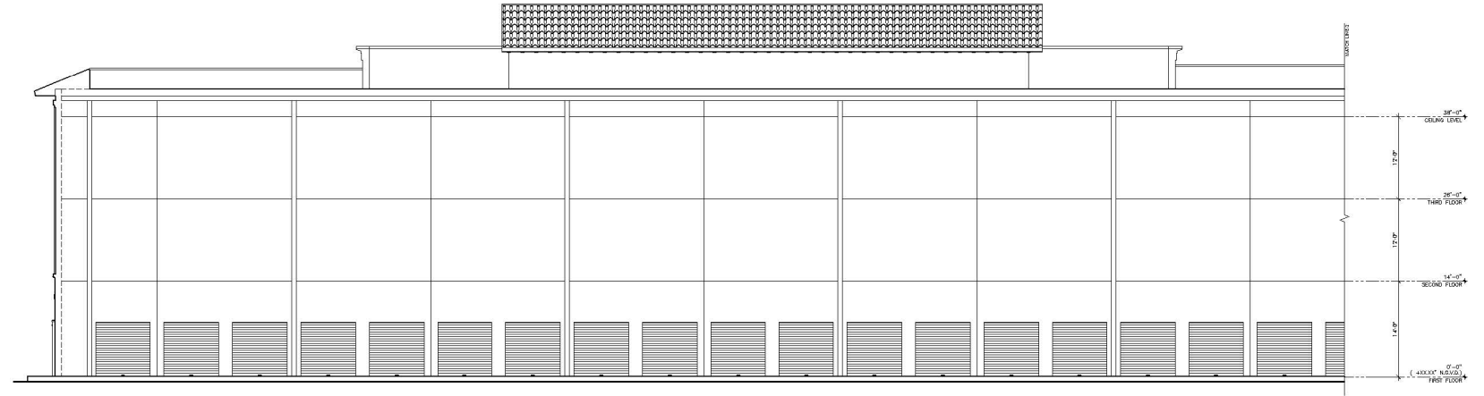
STORAGE BUILDING - NORTH ELEVATION 1/8" = 1'-0"
