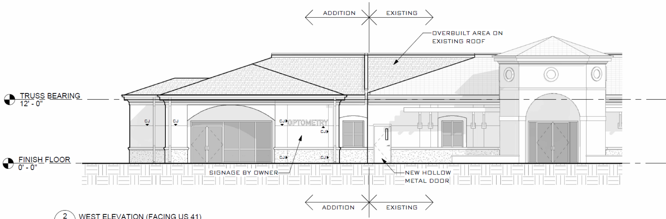
2 WEST ELEVATION (FACING US 41) DO3.0 1/8" = 1'-0"
