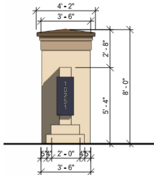
Front Elevation
