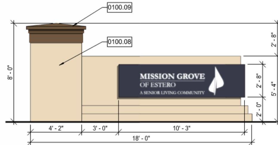
Side Elevation
